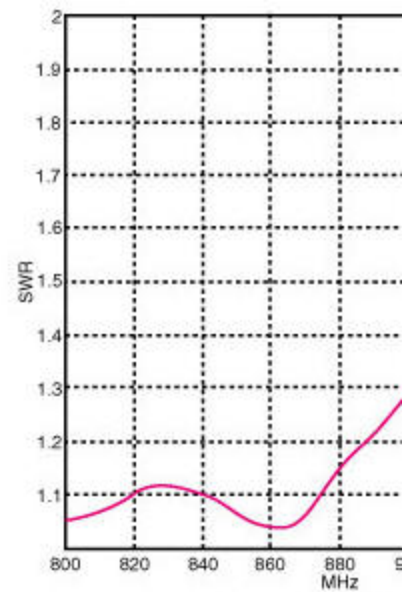
Typical VSWR
